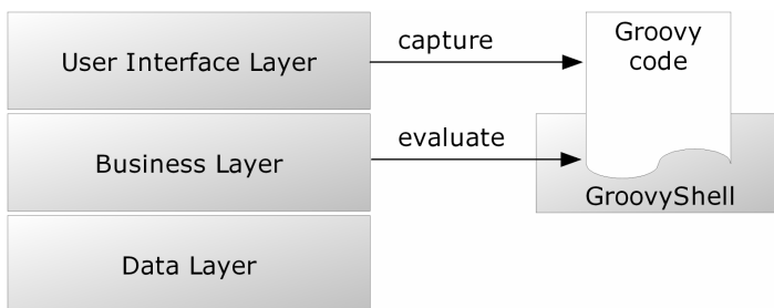
Figure 11.1 One example of an integration solution. Groovy code is entered by the user in the user interface layer and then executed in the business layer.
