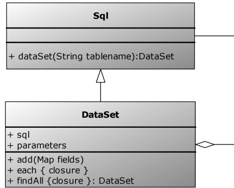
Figure 10.2 UML class diagram of groovy.sql.DataSet decorating groovy.sql.Sql
