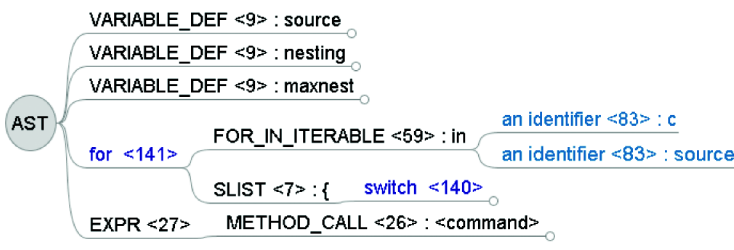
Figure 13.6 Mindmap AST of listing 13.17 expanded on a for loop
